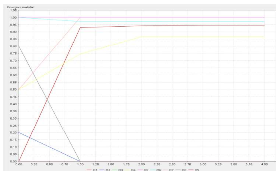
Figure 15: The first convergence visualisation of scenario 4 with IV = [0.0, -1.2, -1.20, 0.5, 1.0, 1.0, 0.50, 0.80]
